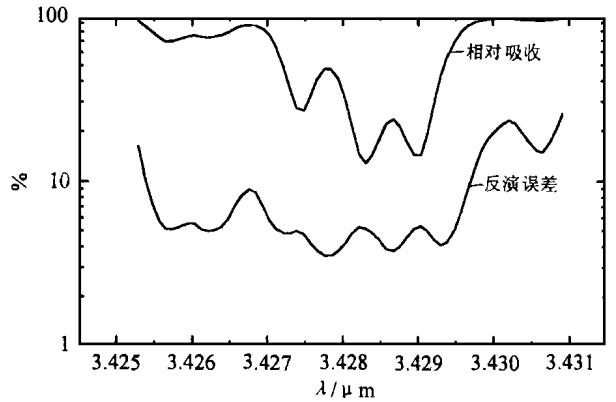
图 4 模拟不同波长上的测量误差对反演结果的影响 Fig. 4 The simulation errors vs. wavelength owing to the measuremental noise, the absorption of this wavelength region is also plotted in the figure
