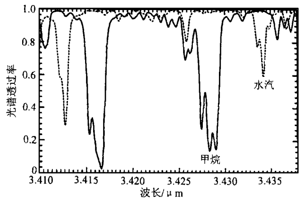
图 1 计算的整层大气中甲烷和水汽的透过率 Fig. 1 Calculated column transmission of atmospheric methane and water vapor
