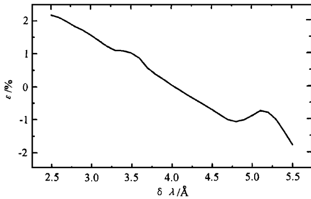
图 3 测量与计算的光谱分辨率的差别对反演结果的影响 Fig. 3 The errors vs. the difference between the calculated and measured spectral resolution
