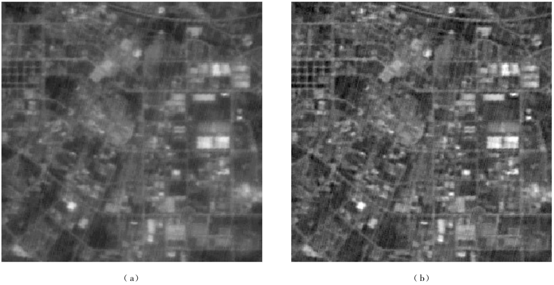
图 3 在大气订正中不考虑邻近像元影响与消除邻近像元影响的结果比较 (a)未考虑邻近像元影响的大气订正结果; (b)考虑邻近像元影响的大气订正结果 Fig 3 Comparison of results between neglecting and correction adjacency effect (a) Image without adjacency correction; (b) Image after adjacency correction
