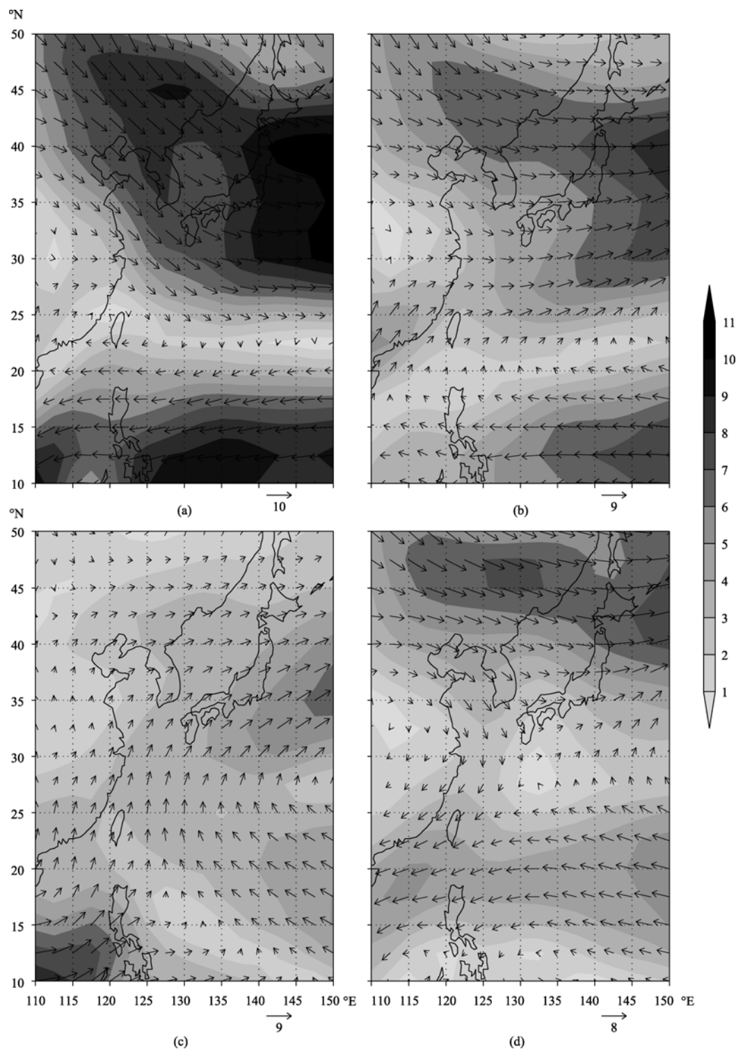
Fig. 9 Sesonal distribution of wind field at 850hp over the China Sea(2000—2006)
