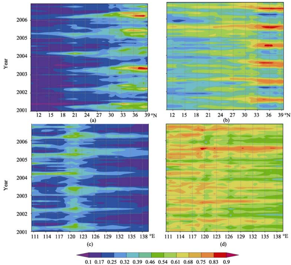
Fig. 7 Meridional and longitudinal distribution of AOT550 and FMF over the China Sea
