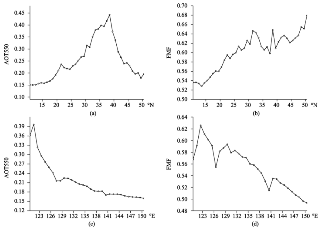
Fig. 8 Meridional and longitudinal distribution of AOT550 and FMF averaged by six years over the China Sea.
