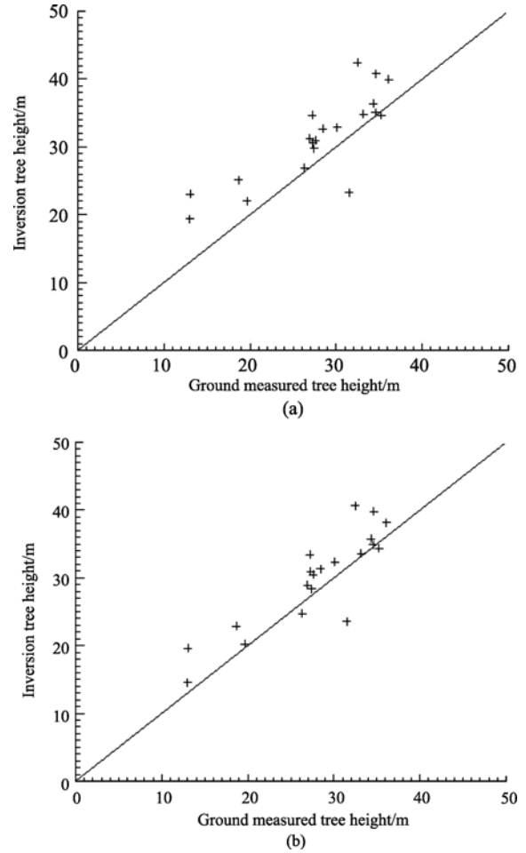
Fig. 9 Scatter diagram of estimated average forest height by the new hybrid inversion method with ground measured average forest height (a) Without non-volumetric decorrelation compensation; (b) With non-volumetric decorrelation compensation
