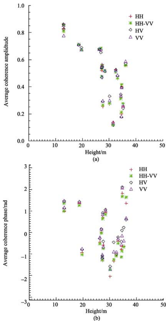
Fig. 2 Scatter diagram of different polarization interferometric coherence vs. forest height (a) Coherence amplitude; (b) Coherence phase
