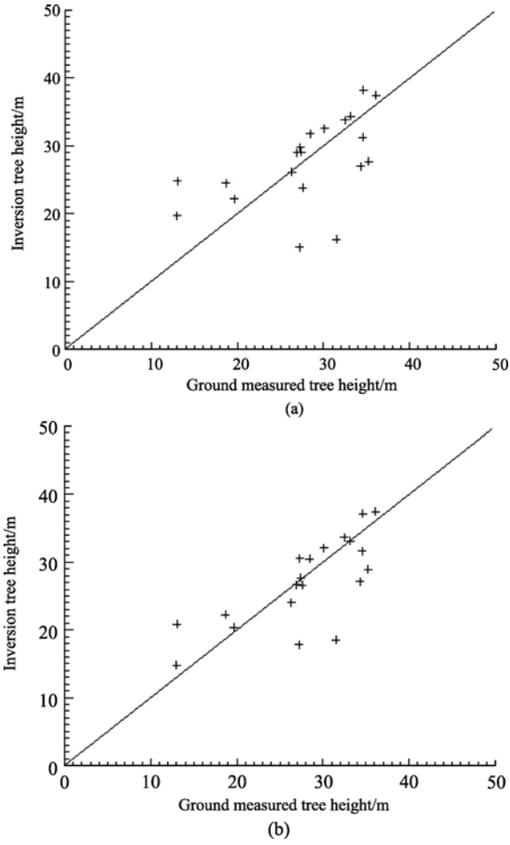
Fig. 8 The scatter diagram of estimated average forest height by the hybrid inversion method with ground measured average forest height (a) Without non-volumetric decorrelation compensation; (b) With non-volumetric decorrelation compensation
