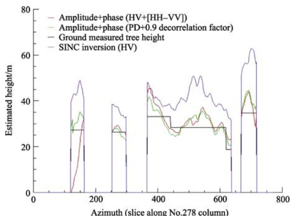
Fig. 10 Forest height profile along the azimuth direction (a straight line of column 278 in the image shown in Fig.1) of three inversion algorithms.
