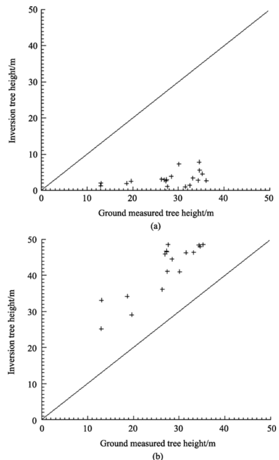
Fig. 4 Scatter diagram of average forest height inverted by DEM difference method with ground measured average forest height. (a) Taking interferometric coherence of HV as \gamma_{w_v} and that of HH-VV as \gamma_{w_s} ; (b) \gamma_{w_v} and \gamma_{w_s} were defined by the PD polarimetric interferometric coherence optimization algorithm
