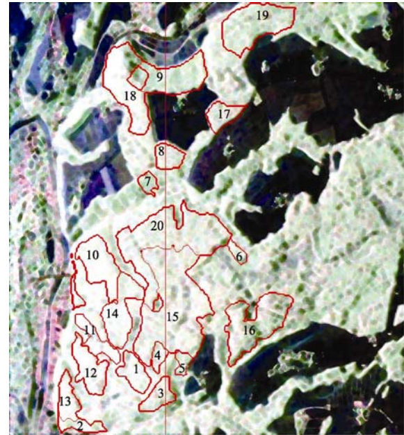
Fig. 1 PAULI decomposition RGB image of the polarimetric SAR data of the test site
