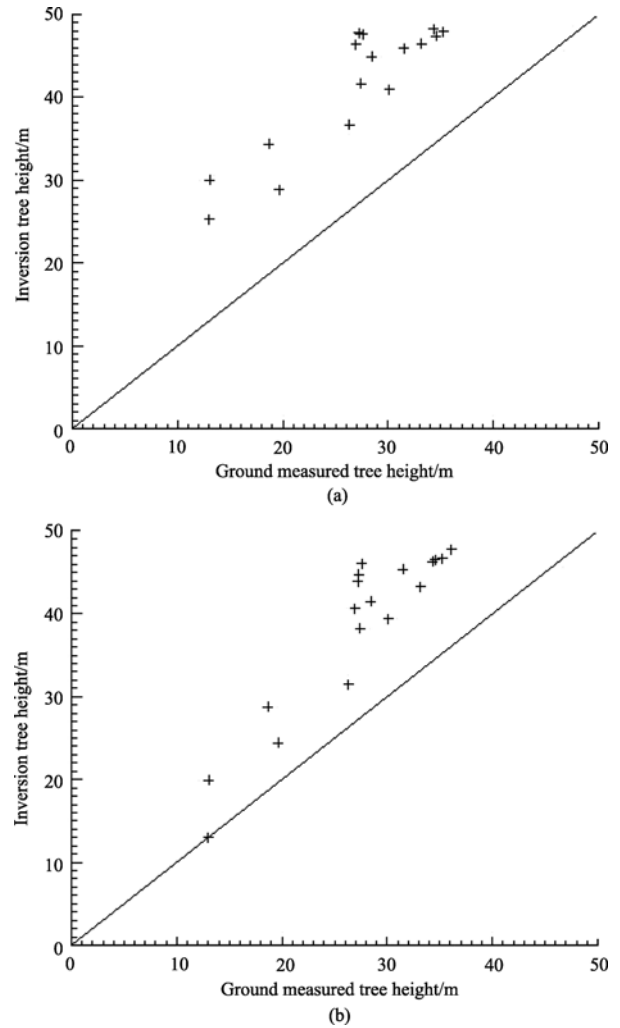
Fig. 6 Scatter diagram of average forest height by SINC inversion model with ground measured average forest height taking HV interferometric coherence as input (a) Without non-volumetric decorrelation compensation; (b) With non-volumetric decorrelation compensation
