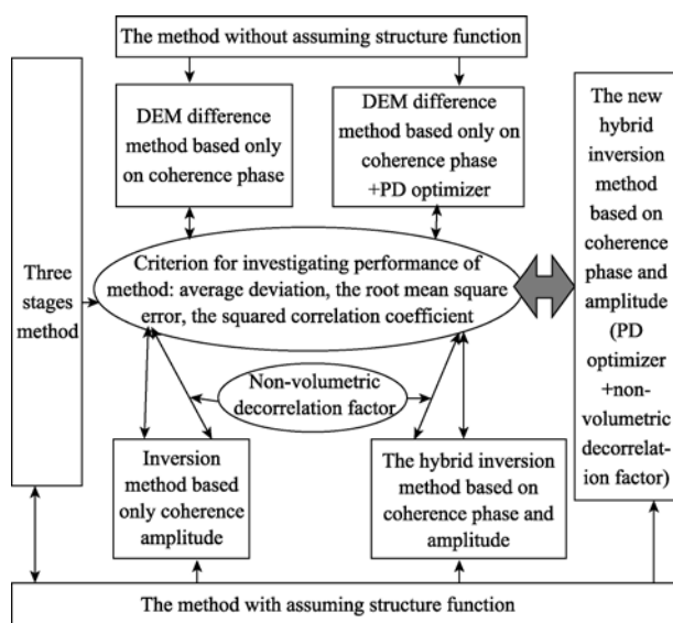
Fig. 3 Flow chart of this study
