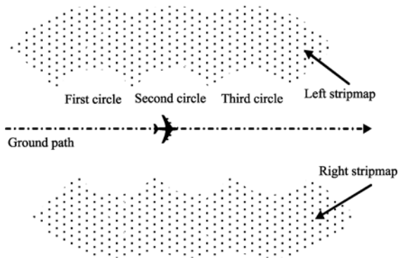
Fig. 2 Sketch map of dual stripmap SAR
