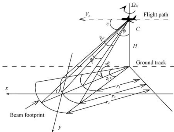
Fig. 4 Circular-scanning SAR data collecting geometry
