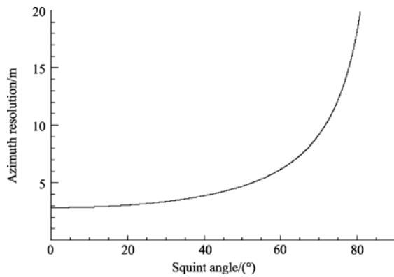
Fig. 7 Relationship curve of azimuth resolution angle
