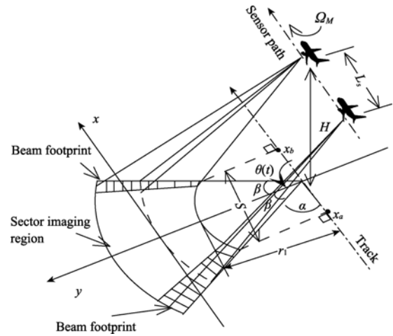
Fig. 8 Formation of imaging region according to and squint the system parameters
