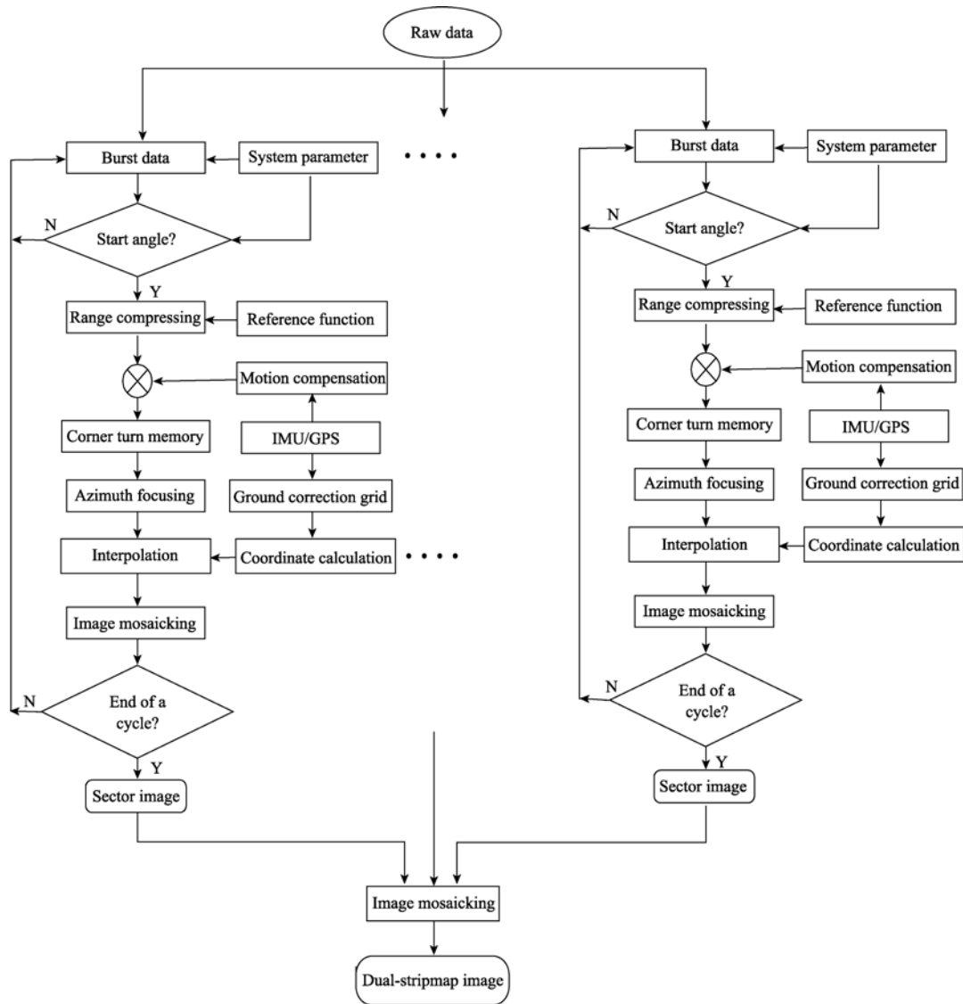
Fig. 6 Signal processing flowchart of the proposed system
