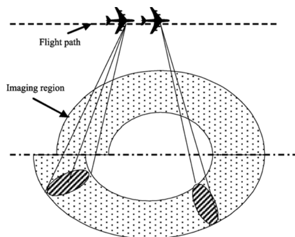
Fig. 1 Sketch map of circular scanning SAR
