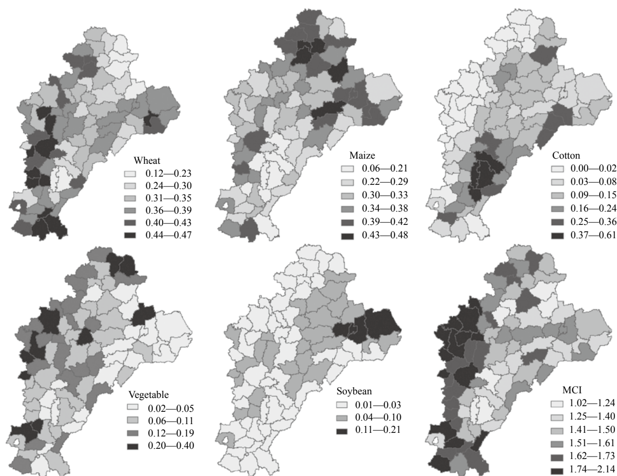
Fig. 7 Ratios of cultivated areas of wheat, corn, cotton, and vegetables to total cultivated area, along with multiple crop index (MCI) for the period of 2002–2007
