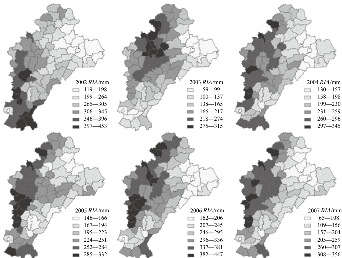
Fig. 2 Distribution of annual required irrigation amount for 2002—2007
