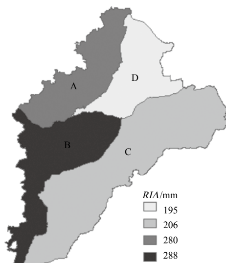
Fig. 4 Annual average irrigation water requirements in different basins (A, B, C, D respectively represent western Daqing River plain, Ziya River plain, Heilonggang plain, eastern Daqing River plain)
