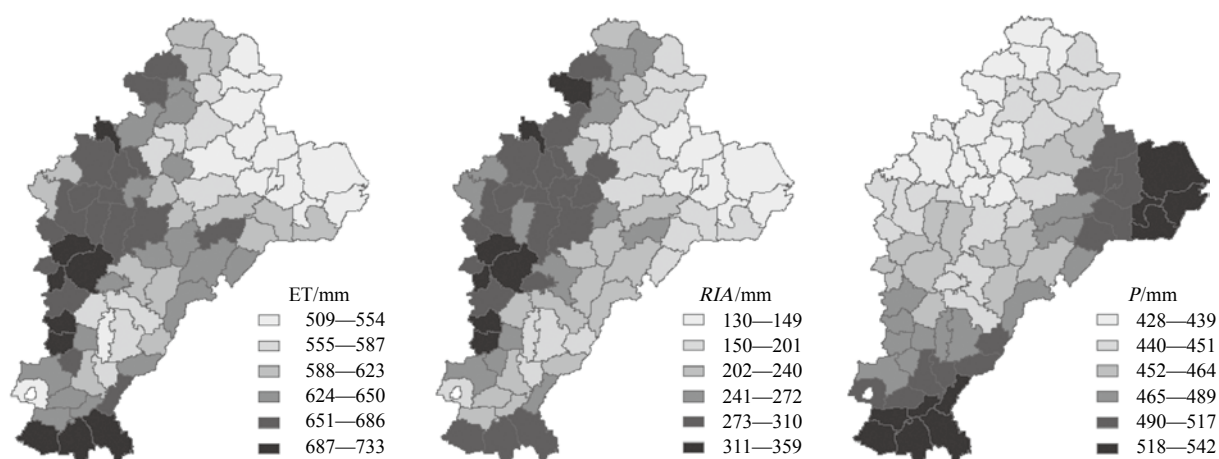
Fig. 5 Plots of distributed annual average evapotranspiration (ET), required irrigation amount (RIA), and precipitation (P)
