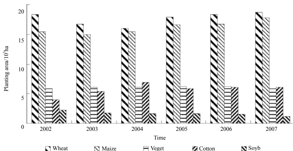
Fig. 6 Variation in cultivated areas of wheat, maize, cotton, vegetables (Veget), and soybean (Soyb) in the study area from 2002 through 2007
