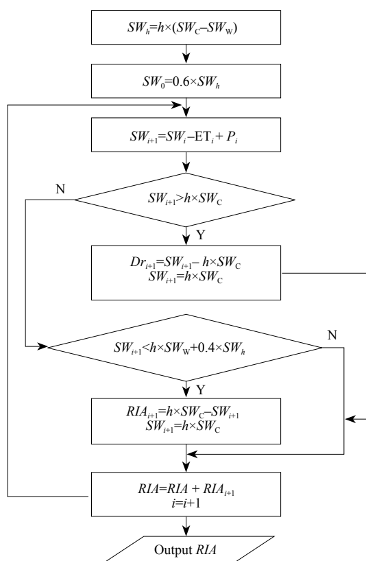
Fig. 1 A schema of irrigation requirement amount computation for the North China Plain study area
