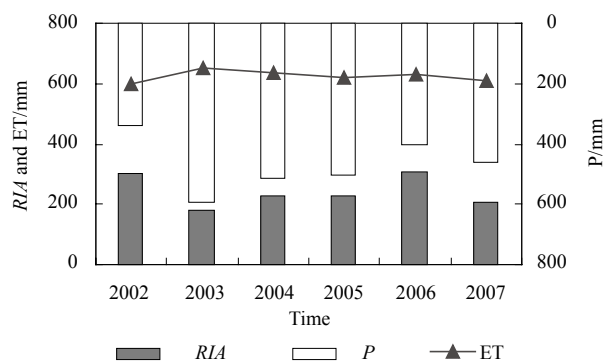
Fig. 3 Comparison of annual required irrigation amount (RIA), precipitation (P), and evapotranspiration (ET) for 2002–2007
