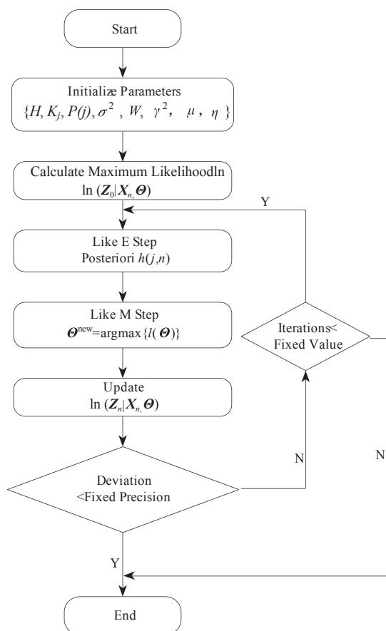
Fig. 6 Training flowchart
