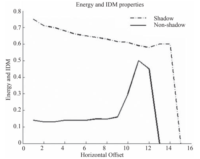
Fig. 5 Analysis of energy and IDM between shadow and non-shadow region
