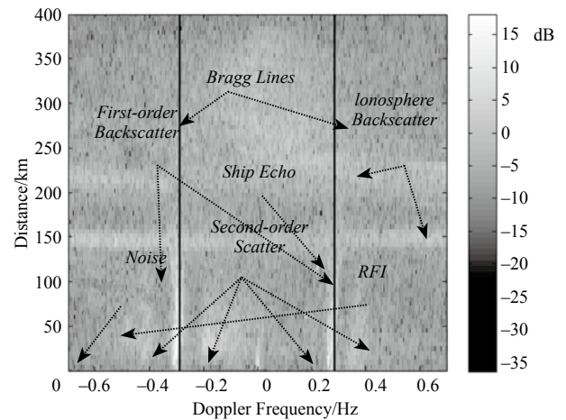
Fig. 2 Range doppler power spectrum of OSMAR071 (12:00, 2008-07-28)
