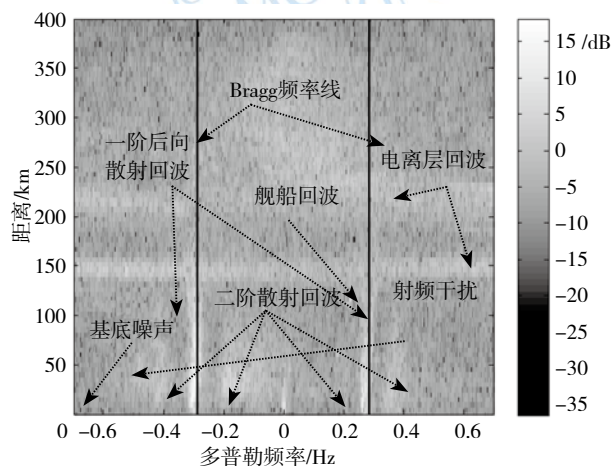
图2 OSMAR071接收的回波多普勒谱 (2008-07-28 T 12:00)
