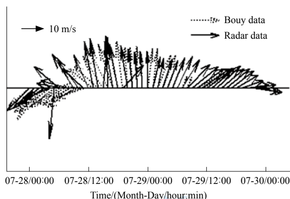
Fig. 8 Comparison of wind vector time series between the radar and buoy (Time: 2008-07-28—29)
