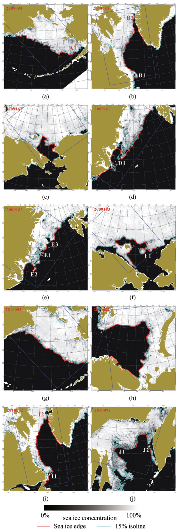
Fig. 6 Comparison between sea ice edge retrieved by changeable image closing operation and the 15% isoline (A—J are the sea ice concentration distribution in different Arctic region, The blue box denotes the range of selected data)
